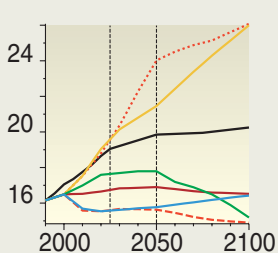
(e) SO 2 emissions (Tg S)
