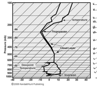
Skew-T Diagram
