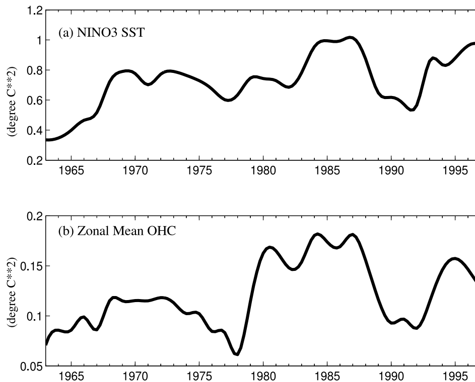
Figure 4. Variance of (a) NINO3 SST and (b) zonal mean OHC calculated within a 10-year window that moves year by year from 1958 to 2001.
