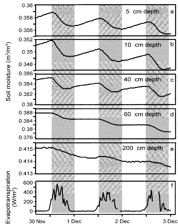
FIG. 3. Soil moisture (30-min means) at (a) 5, (b) 10, (c) 40, (d) 60, and (e) 200 cm beneath the soil surface. (f) Evapotranspiration, measured by eddy covariance. The observations were made during a rain-free period late in the 2000 dry season (30 November–2 December).
