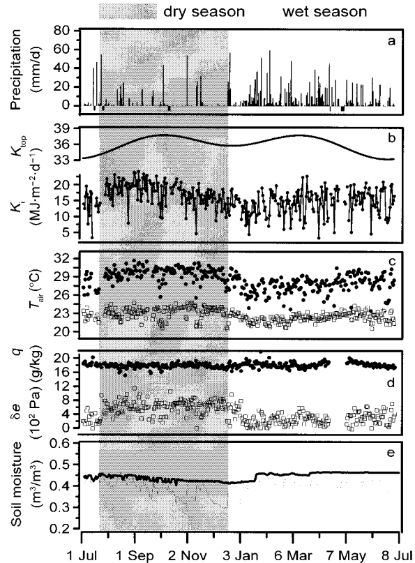
FIG. 1. (a) Daily precipitation at 64 m (negative bars are missing values). (b) Daily mean solar radiation at 64 m ( K_i ; lines connecting filled circles) and calculated daily mean solar radiation at the top of the atmosphere ( K_{top} ; solid line). (c) Maximum (filled circles) and minimum (open squares) air temperature at 64 m. (d) Daily mean specific humidity ( q ; lines connecting filled circles), and daily mean water vapor pressure deficit ( \delta e ; open squares). (Note that the scale for \delta e is in hundreds of pascals.) (e) Daily mean volumetric soil moisture at 5 cm depth (thin solid line) and at 250 cm depth (thick solid line). All data are calculated for 24-h periods from 1 July 2000 to 5 July 2001. The dry season is shaded.
