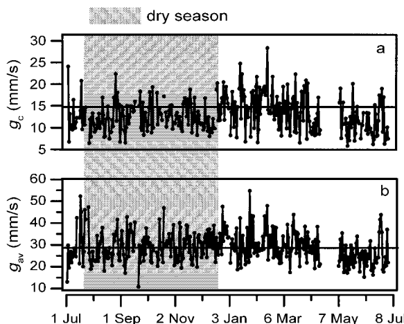
FIG. 9. (a) Surface conductance ( g_c ; 24-h averages connected by lines) and (b) aerodynamic conductance of water vapor ( g_{av} ) from 1 July 2000 to 30 June 2001. The horizontal lines represent the annual means. The dry season is shaded.
