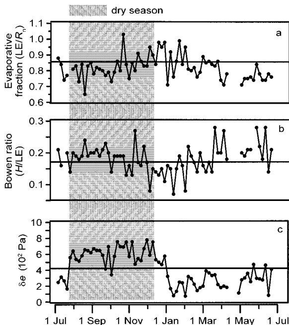
FIG. 8. (a) Evaporative fraction (daytime latent heat flux divided by net radiation; lines connecting 5-d means), (b) Bowen ratio (ratio of daytime sensible heat flux to latent heat flux), and (c) water vapor pressure deficit (note that the scale is in hundreds of pascals). The horizontal lines represent the annual means. The dry season is shaded.
