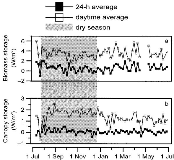
FIG. 6. (a) Biomass energy storage averaged over 24 h (line connecting filled squares for 5-d means) and averaged over the 12 daytime hours (line connecting open squares). (b) Canopy energy storage averaged over 24 h (line connecting filled squares) and averaged over the 12 daytime hours (line connecting open squares). The dry season is shaded.
