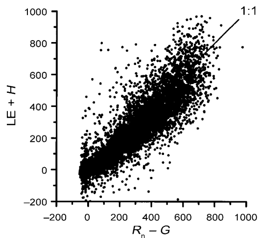
FIG. 5. Available energy (net radiation [ R_n ] minus the sum [ G ] of soil heat flux, biomass heat storage, and canopy heat storage) plotted against the sum of latent (LE) and sensible heat ( H ) flux ( Y = 0.864 X + 10.3 , R^2 = 0.86 , n = 14\,064 points).
