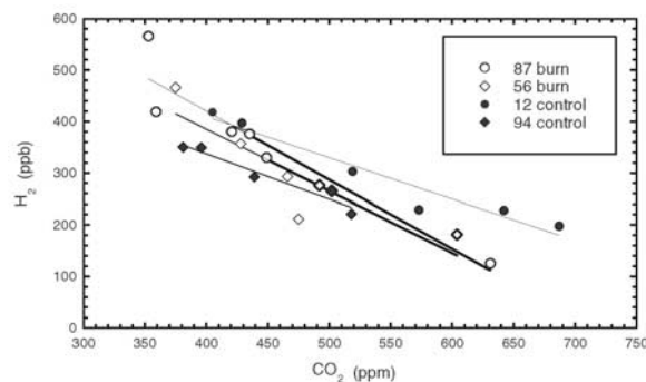
Figure 2. Relationship of H 2 uptake to respired CO 2 observed within the forest canopies during nighttime inversions for the different sites as noted in the legend.
