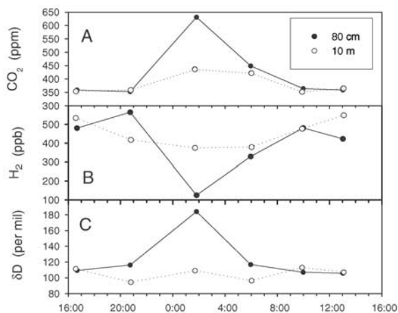
Figure 1. Diel time series collected within (0.8 m) and above (10 m) the forest canopy at burn site 87B. (a) CO 2 concentration (b) H 2 concentration (c) δD of H 2 .
