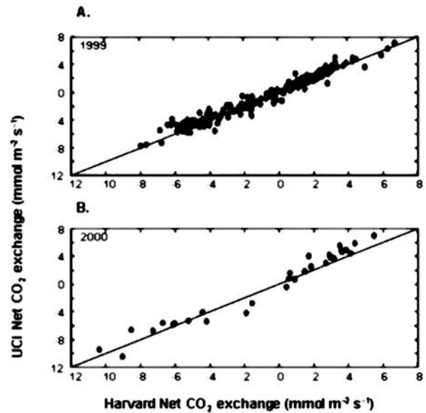
Figure 2. Comparison between 30 min averaged CO 2 fluxes measured by (a) portable system with closed-path IRGA (University of California, Irvine) and fixed tower at NOBS (Harvard) in 1999 and (b) portable system with open-path IRGA (University of California, Irvine) and fixed tower at NOBS (Harvard) in 2000 during system comparisons on NOBS tower. Line in both graphs is 1:1 line.
