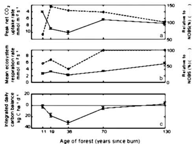
Figure 9. Patterns in measured (a) peak net CO 2 uptake, (b) mean nighttime respiration, and (c) daily carbon balance along chronosequence (solid lines). Error bars are standard errors. Dashed lines in Figures 9a and 9b are percent of measured values in younger burns relative to simultaneous measurements made at NOBS.
