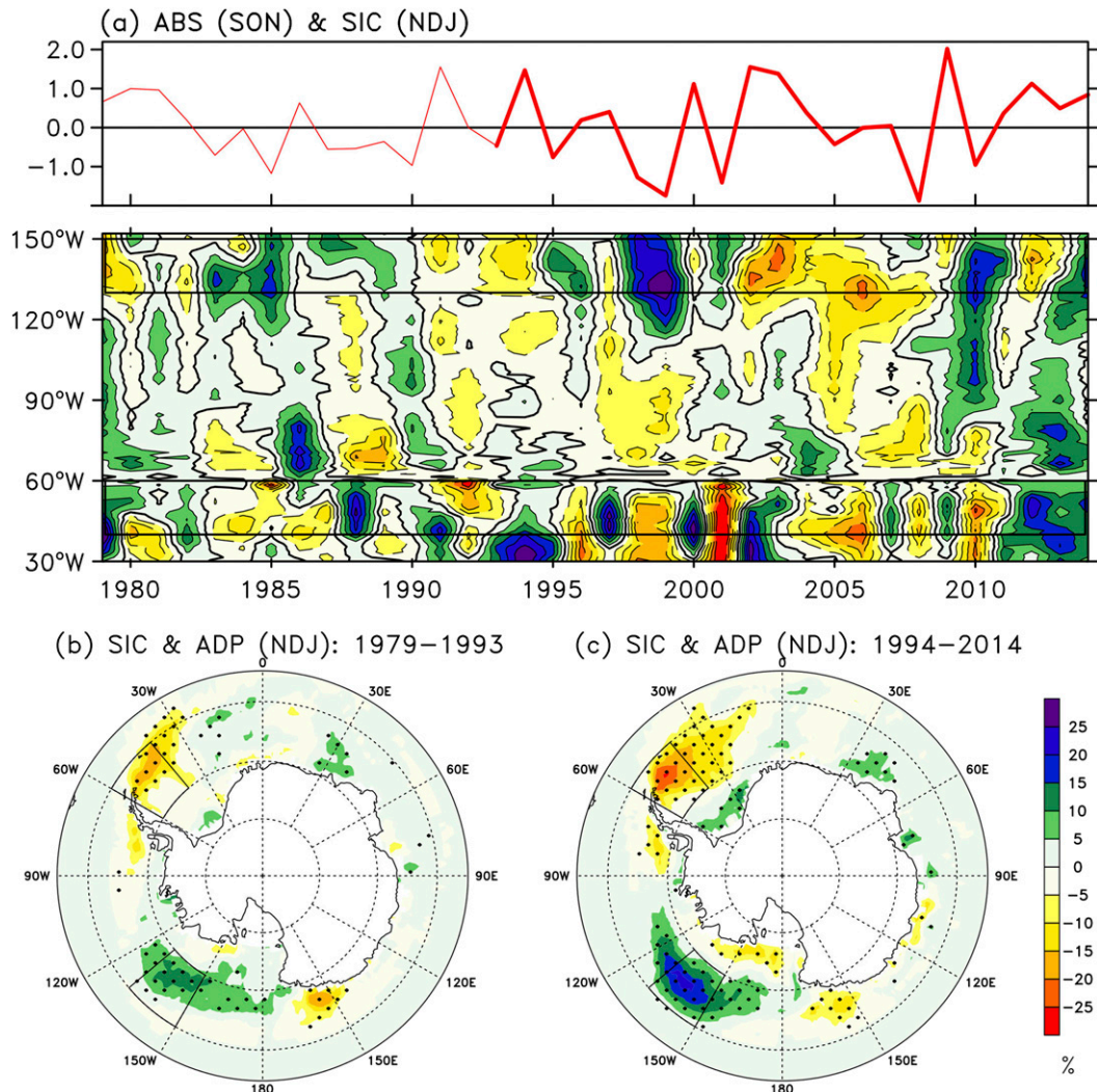
FIG. 10. (a) Time series of the standardized ABS index in SON at top and the longitudinal distribution of SIC anomalies at bottom (%) averaged over 60^{\circ} – 70^{\circ} S in the early summer (NDJ). The thick red line emphasizes the intensified ABS after the early 1990s. Black boxes in the bottom of (a) indicate the Pacific sector (top box; 130^{\circ} – 150^{\circ} W) and Atlantic sector (bottom box; 40^{\circ} – 60^{\circ} W) of the ADP. Regressed SIC anomalies onto the ADP index in NDJ for the periods (b) 1979–93 and (c) 1994–2014. Black boxes in (b),(c) indicate the regions where the ADP index is defined. The areas exceeding the 95% interval determined using a two-tailed Student's t test are dotted.
