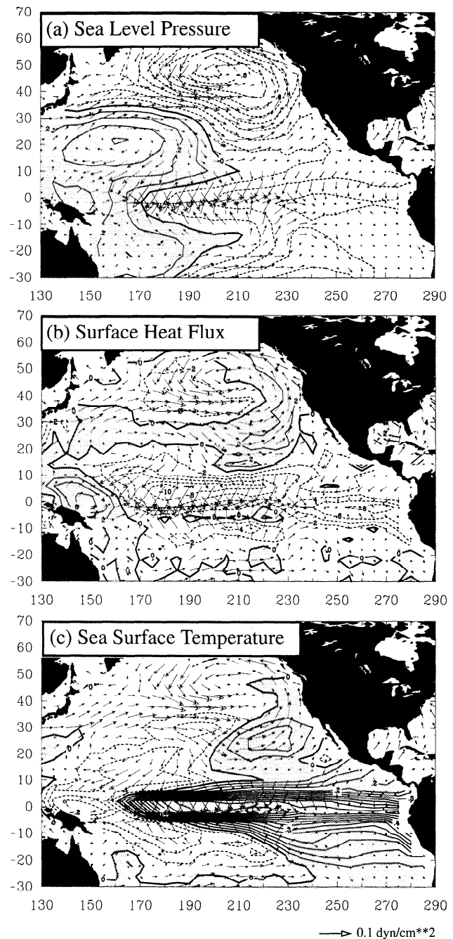
Figure 5. Linear regression coefficients between the principal component of the leading EOF mode of Fig. 2 and anomalies in (a) sea level pressure, (b) surface heat flux, and (c) SST. Vectors represent regression coefficients between the principal component and zonal and meridional wind stress anomalies. Vector magnitudes are in unit of \text{dyn}/\text{cm}^2 . Contours intervals are 0.1\text{mb} for (a), 0.2\text{W}/\text{m}^2 for (b), and 0.05^{\circ}\text{K} for (c). Positive values are shaded. Positive (negative) values in (b) indicate less (more) surface heat flux out of the ocean.
