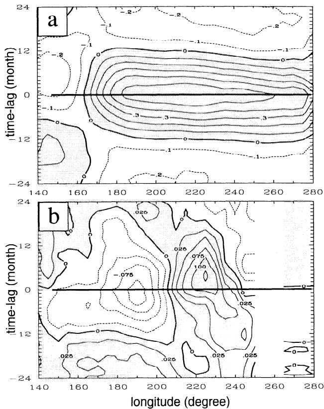
Figure 4. Time-lag regression between the principal component of the leading EOF mode shown in Fig. 2 and SST anomalies (a) at the equator ( 4^{\circ}\text{S}\sim 4^{\circ}\text{N} ) and (b) in the northern subtropics ( 24^{\circ}\text{N}\sim 36^{\circ}\text{N} ). Contour interval is 0.1^{\circ}\text{K} for (a) and 0.025^{\circ}\text{K} for (b).
