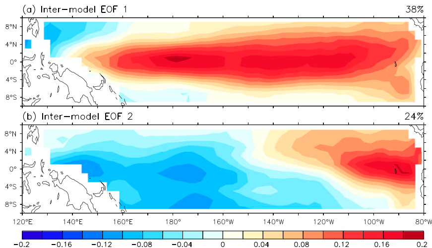
FIG. 6. Leading EOF modes for intermodel variability of the relative centennial warming in the equatorial Pacific ( 10^{\circ}\text{S} – 10^{\circ}\text{N} , 120^{\circ}\text{E} – 80^{\circ}\text{W} ) with the variances they explain calculated from the 18 CMIP5 RCP4.5 simulations.
