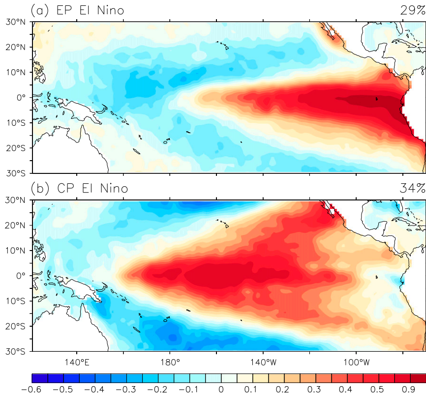
FIG. 1. Observed SST patterns and intensity of the (a) EP and (b) CP types of El Niño with the EOF variances they explain calculated from the HadISST.
