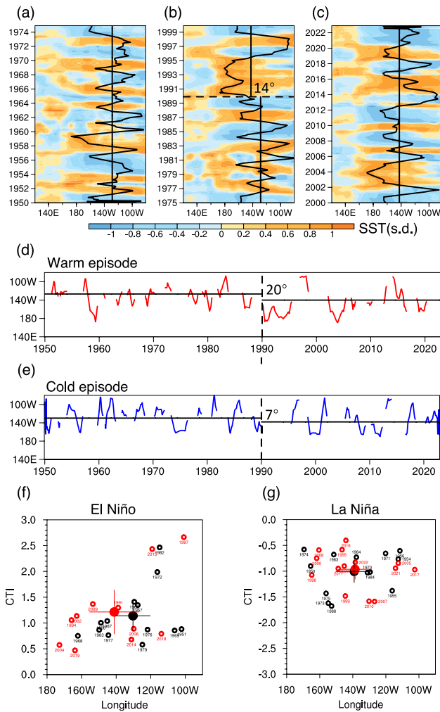
Figure 1. (a–c) Evolution of standardized equatorial (5°S–5°N) SSTA (shading) from 1950 to 2022, smoothed by a 10°-longitude and 10-month running mean. Black lines indicate the longitudinal location of maximum positive (minimum negative) SSTAs over the central-to-eastern Pacific (120°E–80°W). (d–e) Red (blue) lines depict central SSTA locations for warm (cold) episodes in (a–c). Dashed lines in (a–e) separate pre-1990 (1950–1989) and post-1990 (1990–2022) periods. Vertical and horizontal solid-black lines denote mean longitude values of SSTA centers, with numbers indicating specific longitude change values. (f, g) Scatter plot illustrates central location (X-axis) and peak intensity (Y-axis) of winter (ND 0 J 1 ) SSTAs for El Niño and La Niña events. Hollow (solid) circles represent individual events (mean value), with black (red) circles indicating events before (after) 1990. Numbers next to each hollow circle mark the developing year of the ENSO events. Error bars show 95% confidence intervals.
