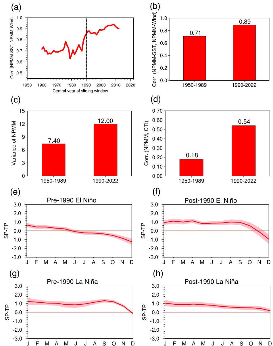
Figure 3. (a) 21-year sliding correlations between FMA 0 NPMM-Wind index and MAM 0 NPMM-SST index. (b) Correlations in (a) separated into pre-1990 and post-1990 periods. (c) Variance of MAM 0 NPMM-SST index in both periods. (d) Correlations between MAM 0 NPMM-SST index and following ND 0 CTI in both periods. Composite difference between standardized SP and TP indices for (e) pre-1990 El Niños and (f) post-1990 El Niños. (g, h) Similar to (e, f), but for La Niñas, with differences multiplied by -1 for relative strength assessment. Pink shading bands represent 95% confidence intervals.
